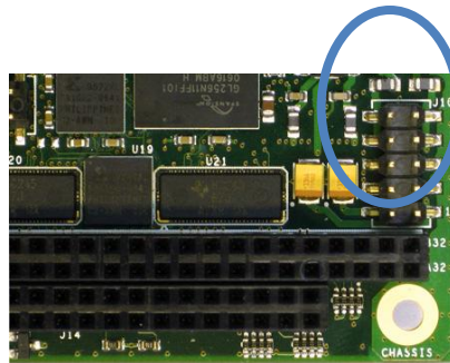
Figure 1: Shown is the 2x5 way vertical USB header that was used on TITAN.
