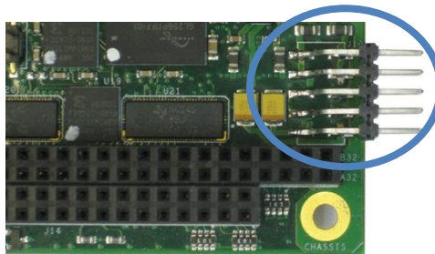
Figure 2: Shown is the 2x5 way right angled header that is being used going forward.
